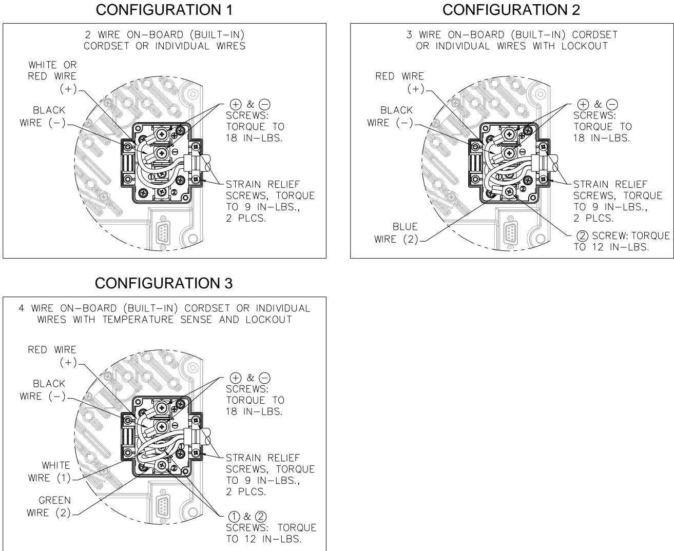
Figure 6.2-4: DC Terminal Block Configurations 1-3
