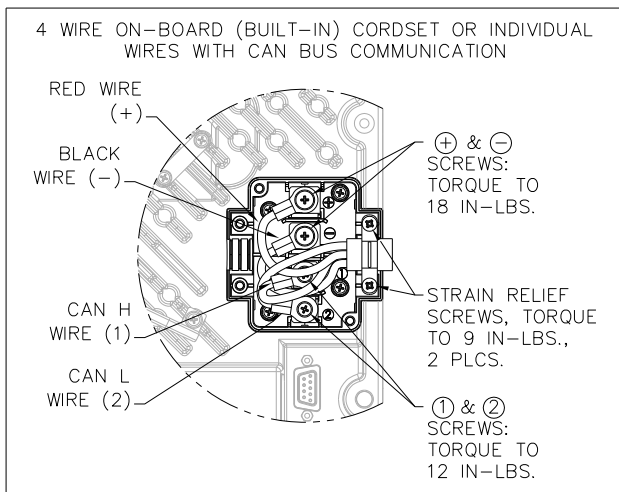
Figure 6.2-4: DC Terminal Block Configurations 4-9
