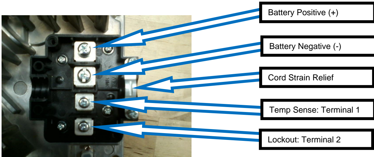
Figure 6.2-1: DC Terminal Block - Models 29300, 29700, 29900, & 30600
