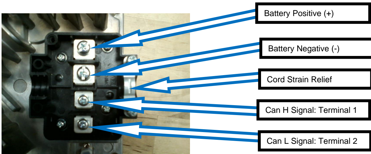
Figure 6.2-2: DC Terminal Block - Models 29310, 29710, 29910, & 30610
