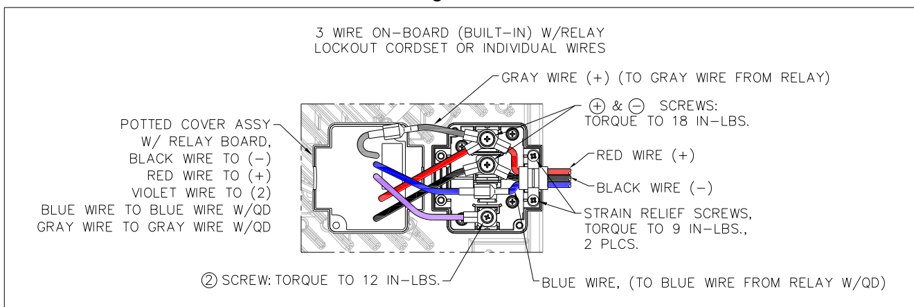
Figure 6.2-4: DC Terminal Block Configurations 10-11
